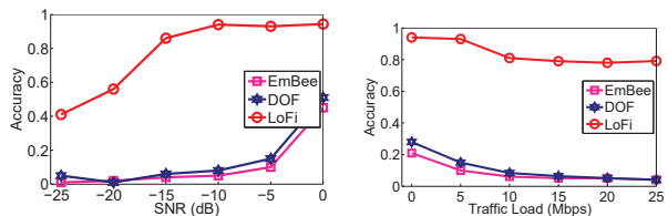
(a) Impact of SNR (5Mbps). (b) Impact of WiFi traffic (-5dB).
