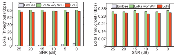
(a) 70Kbps LoRa data rate. (b) 0.486Kbps LoRa data rate.
