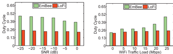
(a) Impact of SNR (25Mbps). (b) Impact of WiFi load (-5dB).
