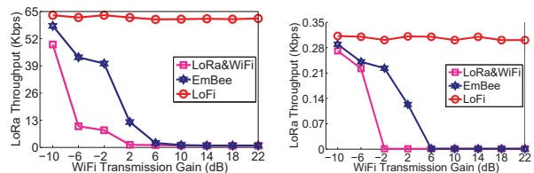
(a) 70Kbps LoRa data rate.
