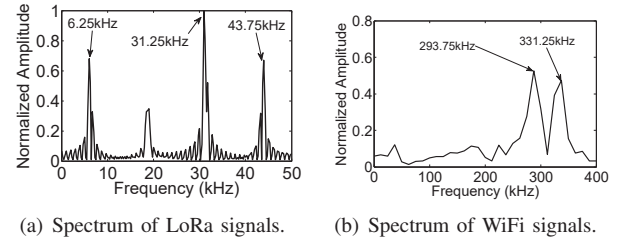
Fig. 7: Spectrum occupancy after multiplication with 18.75kHz signals.
